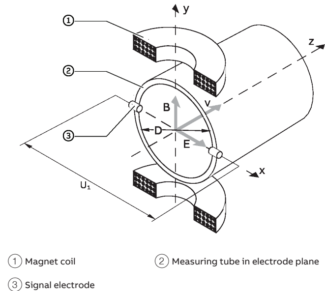
Figure 2 Electromagnetic flowmeter schematic
