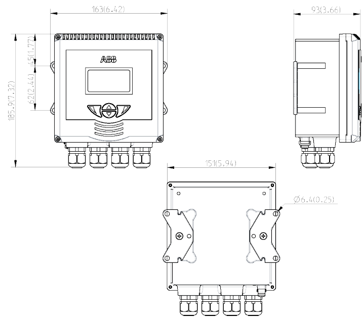
Figure 46 Mounting dimensions (remote mount design)
