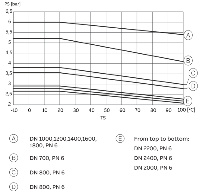
Figure 15 DIN flange, stainless steel, DN 700-2400, PN 6, 1.3 x DN lay length
