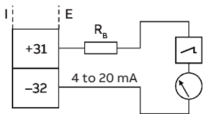
Figure 48 Connection example for active current output 31 / 32 (I = internal, E = external, RB = load)
