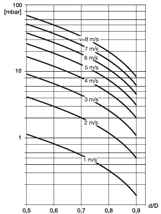
Figure 42 Flow rate nomogram for flange transition piece at \alpha/2 = 8^\circ
