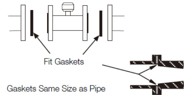
Gasket Fitting
