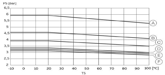
Figure 6 DIN flange, stainless steel, DN 200-600
