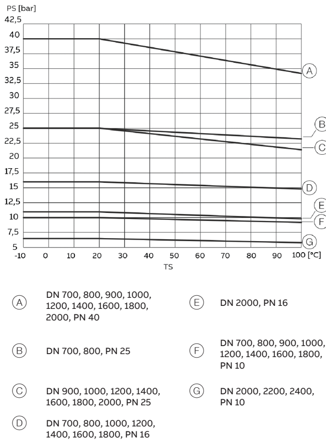
Figure 14 DIN flange, carbon steel, DN 700-2400, PN 10,16,25,40, 1.3 x DN lay length
