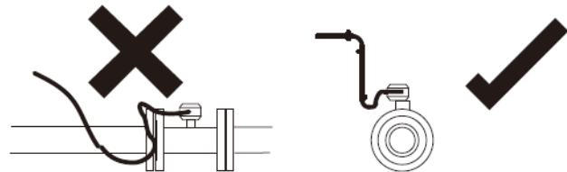
Cable Routing
