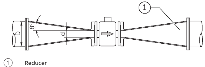
Figure 41 Using reducers
