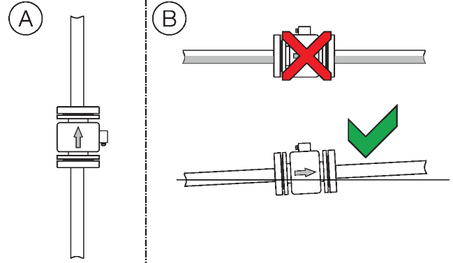
Figure 32 Mounting position
