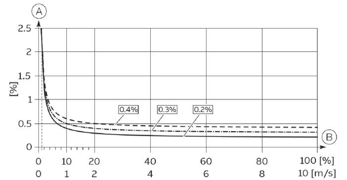
A Accuracy ± of measured value in % B Flow velocity v in m/s, Q / Q max DN in %
