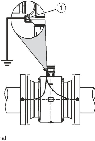
Figure 38 Metal pipe, without liner
