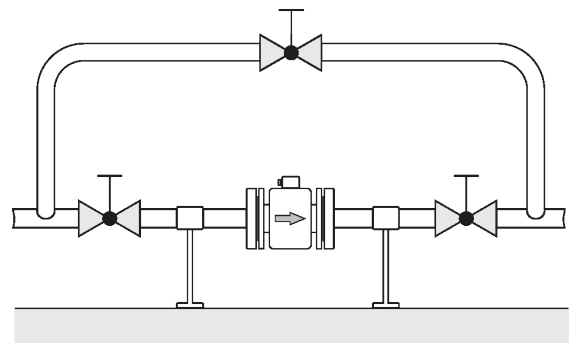
Figure 36 Bypass line
