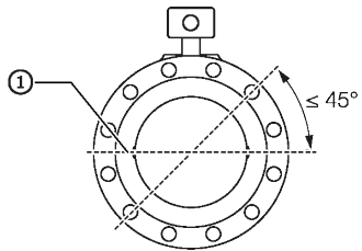
Figure 31 Orientation of the electrode axis
