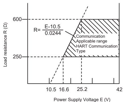
Figure 4 Relationship between power supply voltage and load resistance
